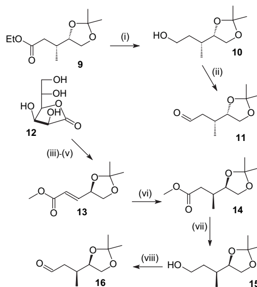
Scheme 4. (i) LiAlH 4 , THF (96%); (ii) PCC (80%); (iii) pyridinium p -toluene sulfonate, 2-methoxypropene, DMF; (iv) NaIO 4 ; (v) methyl diisopropoxyphosphinyl acetate, K 2 CO 3 (34%, three steps); (vi) MeLi, –78 °C (82%); (vii) LiAlH 4 , THF (80%); (viii) PCC (81%).
