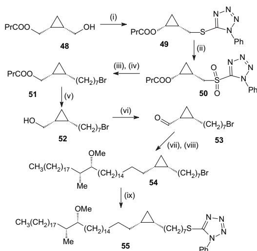
Scheme 13. (i) Diethyl azodicarboxylate, 1-phenyl-1 H -tetrazol-5-thiol, PPh 3 , THF (85%); (ii) H 2 O 2 , Mo 7 O 24 (NH 4 ) 6 ·4H 2 O, IMS (93%); (iii) LiHMDS, THF, 6-bromohexanal (74%); (iv) 2,4,6-triisopropyl sulfonylhydrazide, THF (80%); (v) K 2 CO 3 , MeOH (85%); (vi) PCC (76%); (vii) LiHMDS, 36 , THF (74%); (viii) 2,4,6-triisopropyl sulfonylhydrazide, THF (80%); (ix) 1-phenyl-1 H -tetrazol-5-thiol, K 2 CO 3 (88%).
