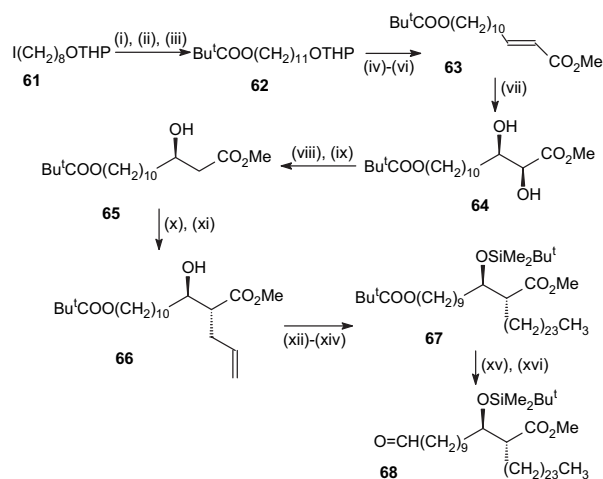
Scheme 15. (i) Li, NH 3 , prop-2-yn-1-ol (94%); (ii) NaBH 4 , Ni(OAc) 2 , EtOH, H 2 (83%); (iii) pivaloyl chloride, Et 3 N, DMAP (91%); (iv) p TsOH, MeOH, THF (89%); (v) PCC (8%); (vi) Ph 3 PCHCO 2 Me, toluene (85%); (vii) (DHQD) 2 -PHAL, K 3 Fe(CN) 6 , K 2 CO 3 , OsO 4 , MeSO 2 NH 2 , Bu t OH, H 2 O (97%); (viii) SOCl 2 , CCl 4 , NaIO 4 , RuCl 3 ·H 2 O (93%); (ix) NaBH 4 , DMAC, THF, H 2 O, H 2 SO 4 (68%); (x) LDA, allyl iodide, HMPA (55%); (xi) imidazole, DMF, TBDMSCl (91%); (xii) OsO 4 , lutidine, NaIO 4 , dioxane, H 2 O (93%); (xiii) LiHMDS, 5-docosan-1-sulfonyl-1-phenyl-1 H -tetrazole (83%); (xiv) H 2 , Pd/C (87%); (xv) KOH, THF, MeOH, H 2 O (80%); (xvi) PCC (84%).
