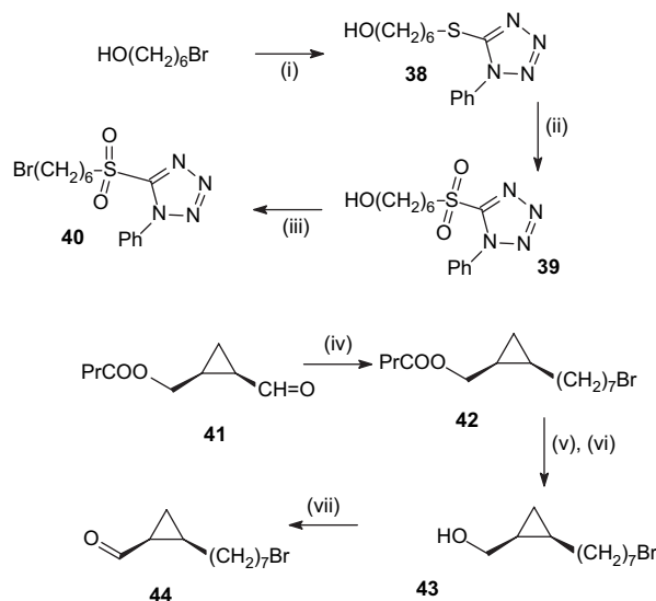
Scheme 10. (i) 1-Phenyl-1 H -tetrazol-5-thiol, \text{K}_2\text{CO}_3 (99.5%); (ii) \text{H}_2\text{O}_2 , \text{Mo}_7\text{O}_{24}(\text{NH}_4)_6 \cdot 4\text{H}_2\text{O} , IMS (90%); (iii) N -bromosuccinimide, \text{PPh}_3 (86%); (iv) LiHMDS, THF, 40 (78%); (v) 2,4,6-triisopropylbenzene sulfonylhydrazide, THF (67%); (vi) \text{K}_2\text{CO}_3 , MeOH (84%); (vii) PCC (93%).
