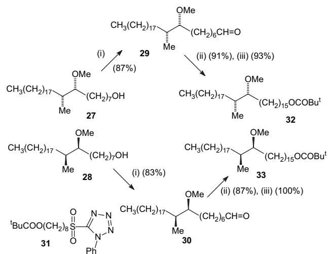
Scheme 8. (i) PCC; (ii) 31 , LiHMDS; (iii) \text{H}_2 , Pd/C.
