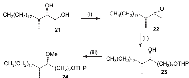
Scheme 6. (i) NaOH, cetrimide, p TsCl, \text{CH}_2\text{Cl}_2 (97%); (ii) \text{BrMg}(\text{CH}_2)_6\text{OTHP} , CuI, THF (75%); (iii) NaH, THF, MeI (94%).
