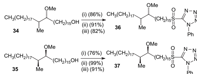
Scheme 9. (i) N -Bromosuccinimide, \text{PPh}_3 , \text{CH}_2\text{Cl}_2 ; (ii) 1-phenyl-1 H -tetrazol-5-thiol, \text{K}_2\text{CO}_3 ; (iii) \text{H}_2\text{O}_2 , \text{Mo}_7\text{O}_{24}(\text{NH}_4)_6 \cdot 4\text{H}_2\text{O} , IMS.
