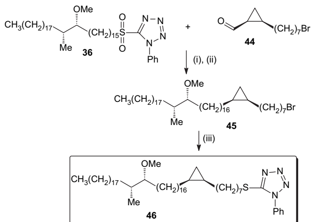
Scheme 11. (i) LiHMDS, THF (92%); (ii) triisopropylbenzene sulfonylhydrazide, THF (91%); (iii) 1-phenyl-1 H -tetrazol-5-thiol, K 2 CO 3 (91%).
