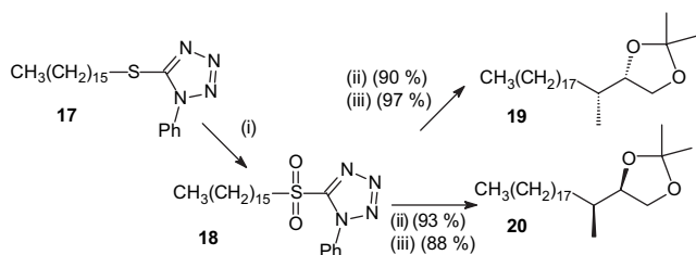
Scheme 5. (i) \text{H}_2\text{O}_2 , \text{Mo}_7\text{O}_{24}(\text{NH}_4)_6 \cdot 4\text{H}_2\text{O} , IMS (93%); (ii) LiHMDS, 16 (for 20 ) or 11 (for 19 ); (iii) \text{H}_2 , Pd/C.
