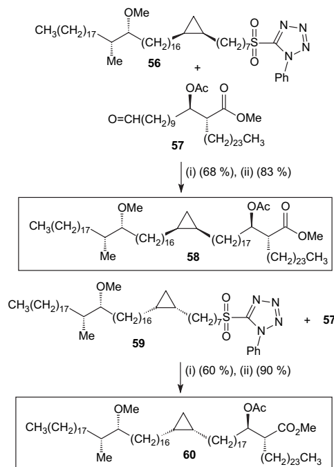
Scheme 14. LiHMDS, THF; (ii) KOOCCN=NCOOK, AcOH, MeOH, THF.
